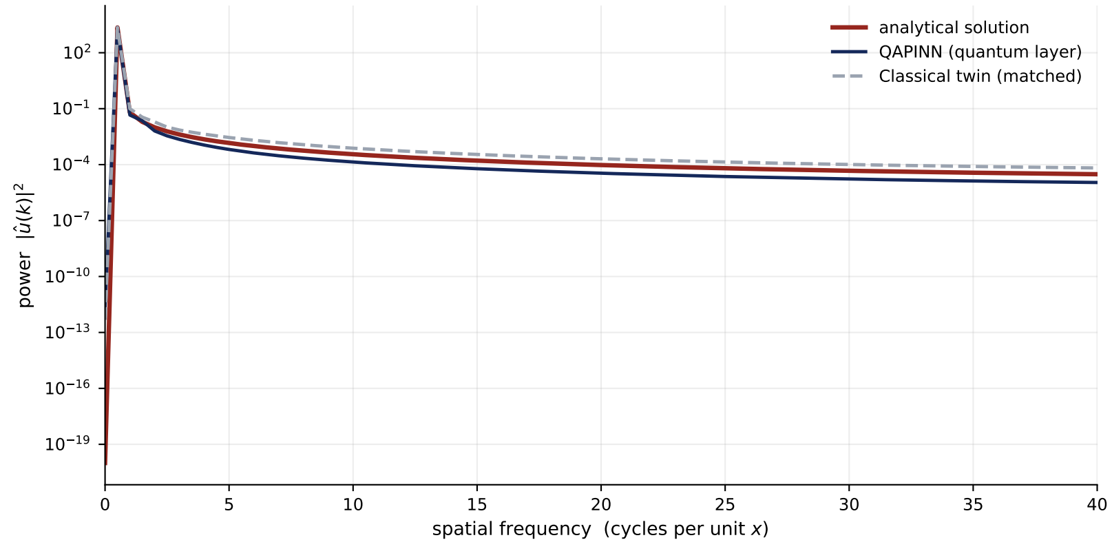
Output Fourier spectrum - heat_n3, t = 1.00 (seed 1234)
